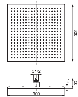
Bloc Overhead Shower
