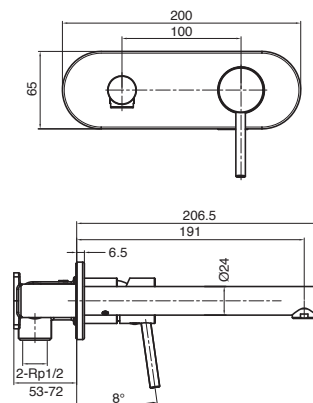
Drift MK2 Wall Basin Mixer Set
