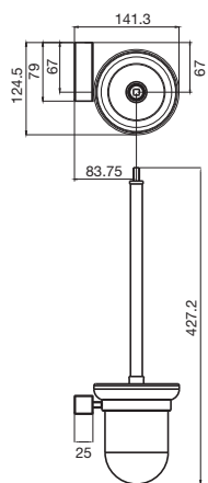
Bloc Toilet Brush and Holder
