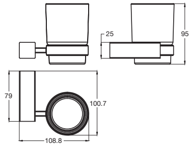
Bloc Glass Tumbler
