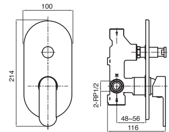
Soothe Shower Mixer with Diverter
