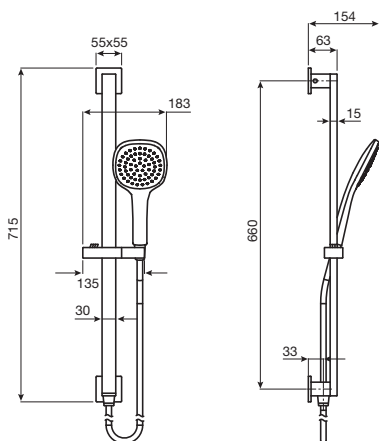
Bloc Single Waterrail Shower
