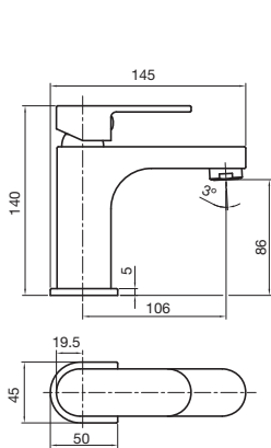
Soothe Basin Mixer
