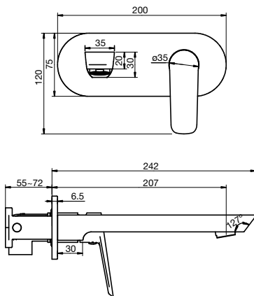
Bliss Wall Basin Mixer Set
