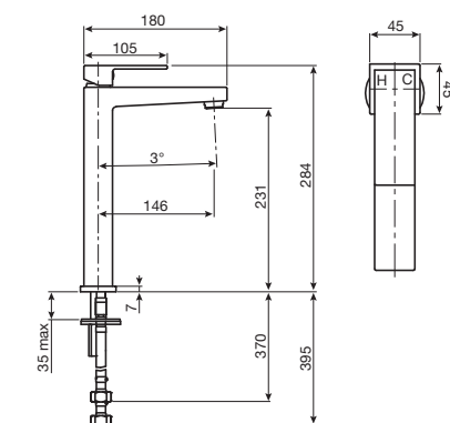
Bloc Extended Basin Mixer
