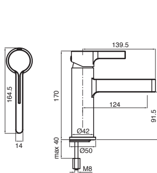
Stream Basin Mixer
