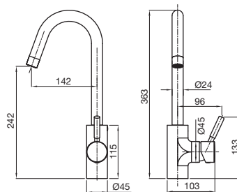
Drift Gooseneck Sink Mixer
