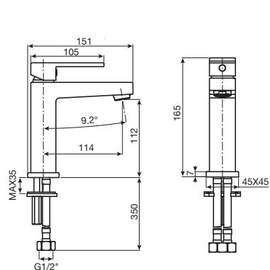
Bloc Basin Mixer
