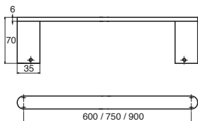
Soothe Single Towel Rail
