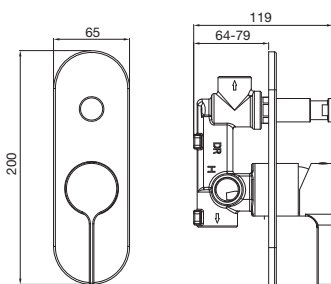
Stream Shower Mixer with Diverter
