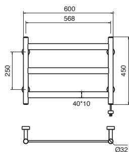
Stream Heated Towel Rail
