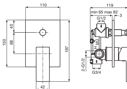
Bloc Shower Mixer with Diverter
