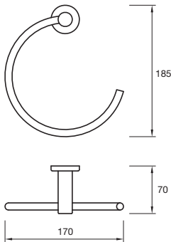
Drift Towel Ring
