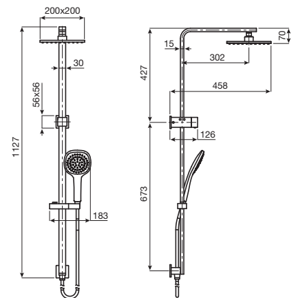
Bloc Twin Waterrail Shower
