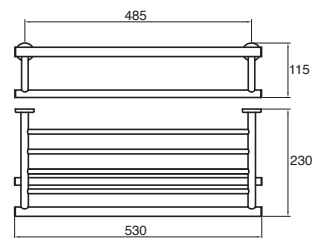
Drift Towel Rack
