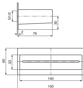
Bloc Waterfall Bath Outlet
