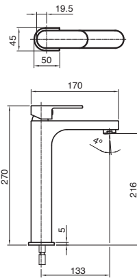
Soothe Extended Basin Mixer
