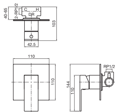
Bloc Shower Mixer
