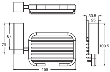
Bloc Soap Basket
