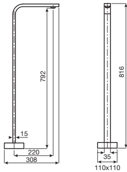
Bloc Floor Bath Outlet
