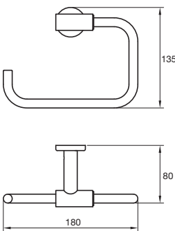
Drift Square Guest Towel Holder
