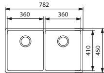
BOW BXX 220-36/36
