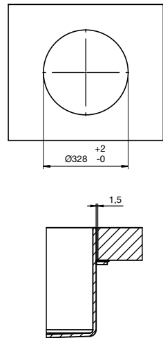
Unisono 325 Flush Mounted Basin No taphole 9506192
