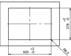
Metaphor 500 Flush Mounted Basin No taphole 9506197
