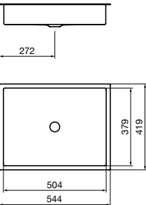
Metaphor 500 Under Counter Basin No taphole 9506282
