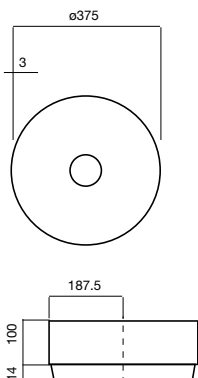
Unisono Counter Basin 375 No taphole 9503960
