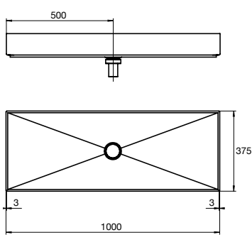
Metaphor 1000 Counter Basin No taphole 9502688
