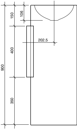
Round Washstand 325 No taphole 1805905
