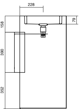
Square Washstand 450 No taphole 9502691
