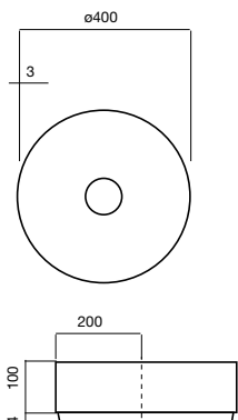
Unisono Counter Basin 400 No taphole 9503959 Also available: Bi-Colour 9508141
