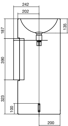
Round Washstand 400 No taphole 9502690 Also available: Freestanding 950327 Bi-Colour 9508140 Dark Iron 9508139
