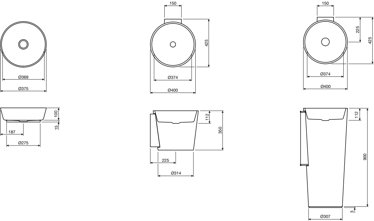
Scpio 375 Counter Basin No taphole 9508133 Also available: Bi-Colour 9508135 Dark Iron 9508134
