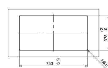
Metaphor 750 Semi Inset Basin No taphole 9506200
