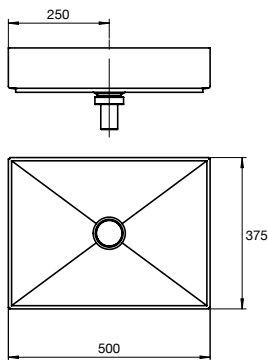
Metaphor 500 Counter Basin No taphole 9502483
