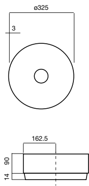
Unisono Counter Basin 325 No taphole 9503961
