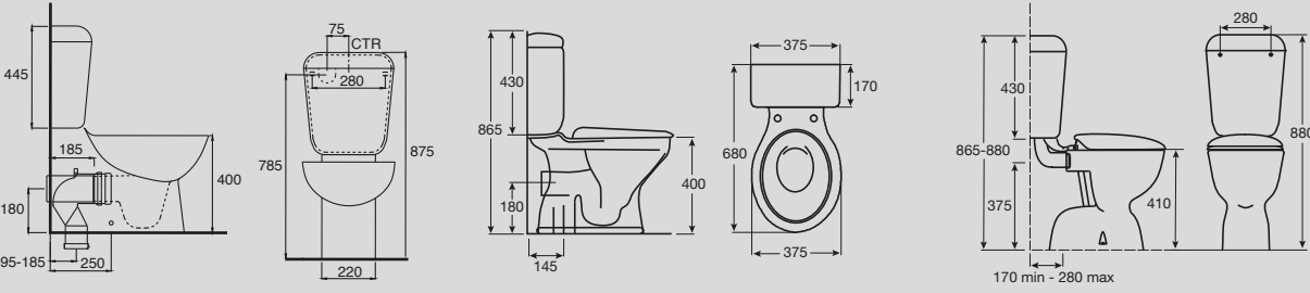
Solus Round Close Coupled Back to Wall Toilet Suite
