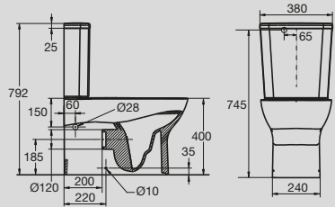
Domaine Close Coupled Back to Wall Rimless Toilet Suite
