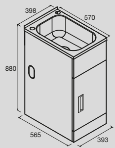
Domaine 27 Litre Laundry Trough and Cabinet
