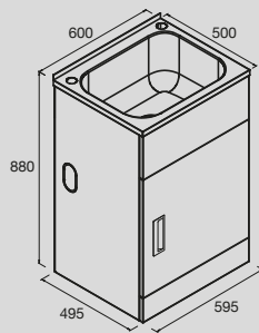
Domaine 45 Litre Laundry Trough and Cabinet
