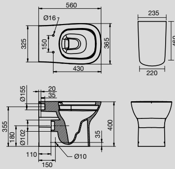
Domaine Back to Wall Rimless Toilet Pan
