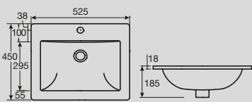
Solus Vanity Basin 525 x 450mm
