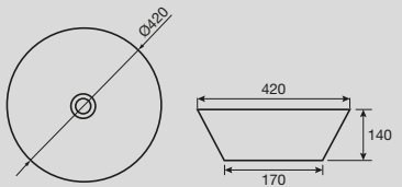
Solus Vessel Basin 420mm
