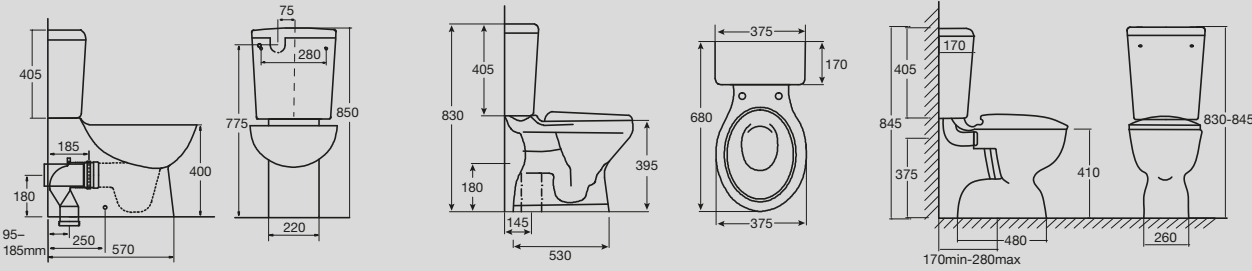
Solus Square Close Coupled Back to Wall Toilet Suite
