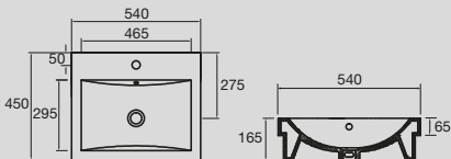
Solus Semi Inset Basin 540 x 450mm
