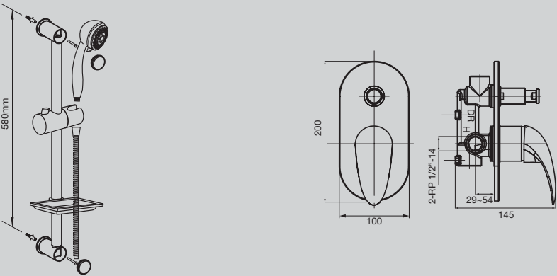
Bristol Rail Shower
