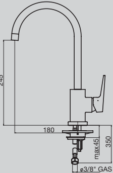
Solus MK2 Gooseneck Sink Mixer
