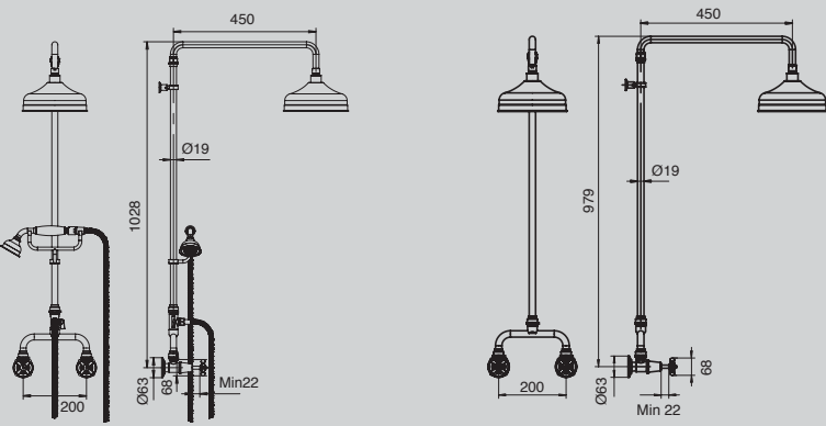
Canterbury Exposed Twin Telephone Shower Set
