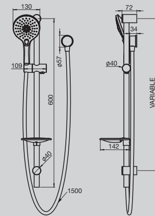
Domaine 3 Function Rail Shower
