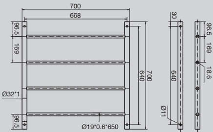
Solus MK2 Heated Towel Rail 700mm h x 700mm w
