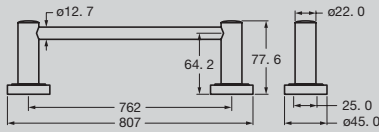
Solus MK2 Single Towel Rail
