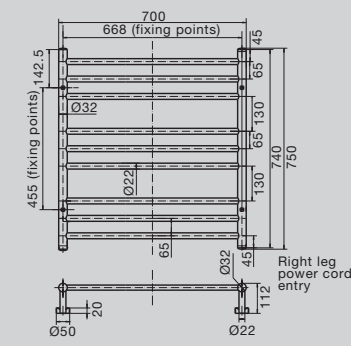
Domaine Heated Towel Rail 750mm h x 700mm w
