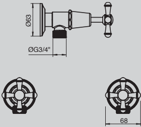
Canterbury Washing Machine Stops
