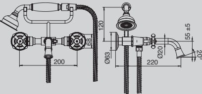
Canterbury Wall Mounted Telephone Bath Shower Set
