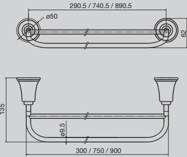
Canterbury Double Towel Rail 300mm / 750mm / 900mm
